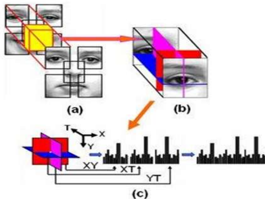
Fig. 3 - Description of facial expressions with local binary patterns [13]
